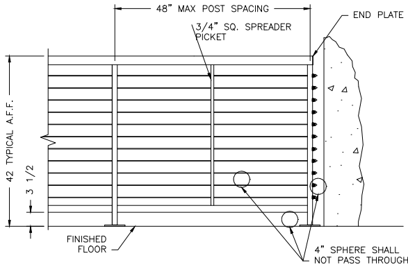
— TYPICAL ELEVATION
