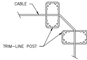
— CORNER DETAIL SCALE: 6
